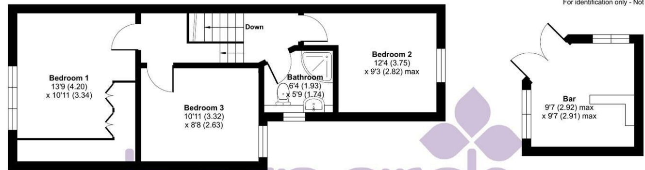
FIRST FLOOR
